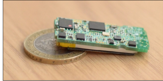
Figure 1. SPW-2: CC2650 based wearable accelerometer sensor [5].
