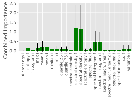
Figure 6. The importance (y-axis) of each feature (x-axis) as determined from the Random Forest (RF) classifier. Errorbars show standard deviation.
